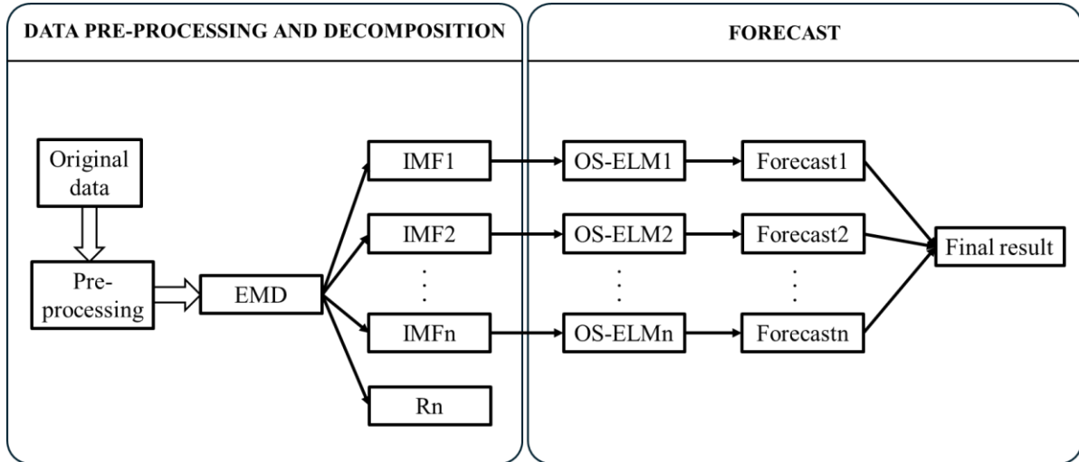
Figure 3: Construction of the proposed model
