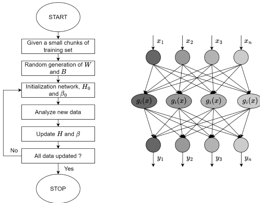
Figure 2: Illustration of OS-ELM structure
