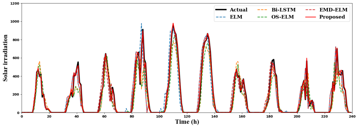
Figure 6: Time-series forecasting results comparison (24-step forecasting)
