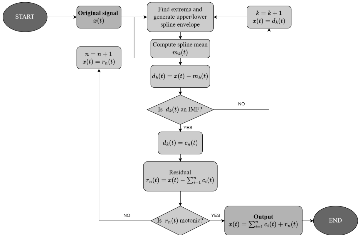
Figure 1: The flowchart of EMD method
